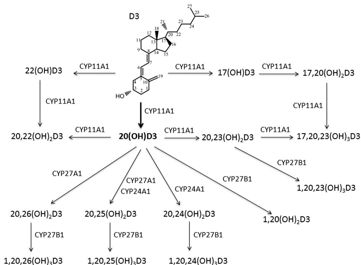
Fig. 1. Summary of the major pathways for metabolism of vitamin D3 by CYP11A1 and the role of CYP27A1, CYP27B1 and CYP24A1 in the further hydroxylation of products. See the text for published references to the reactions listed.
