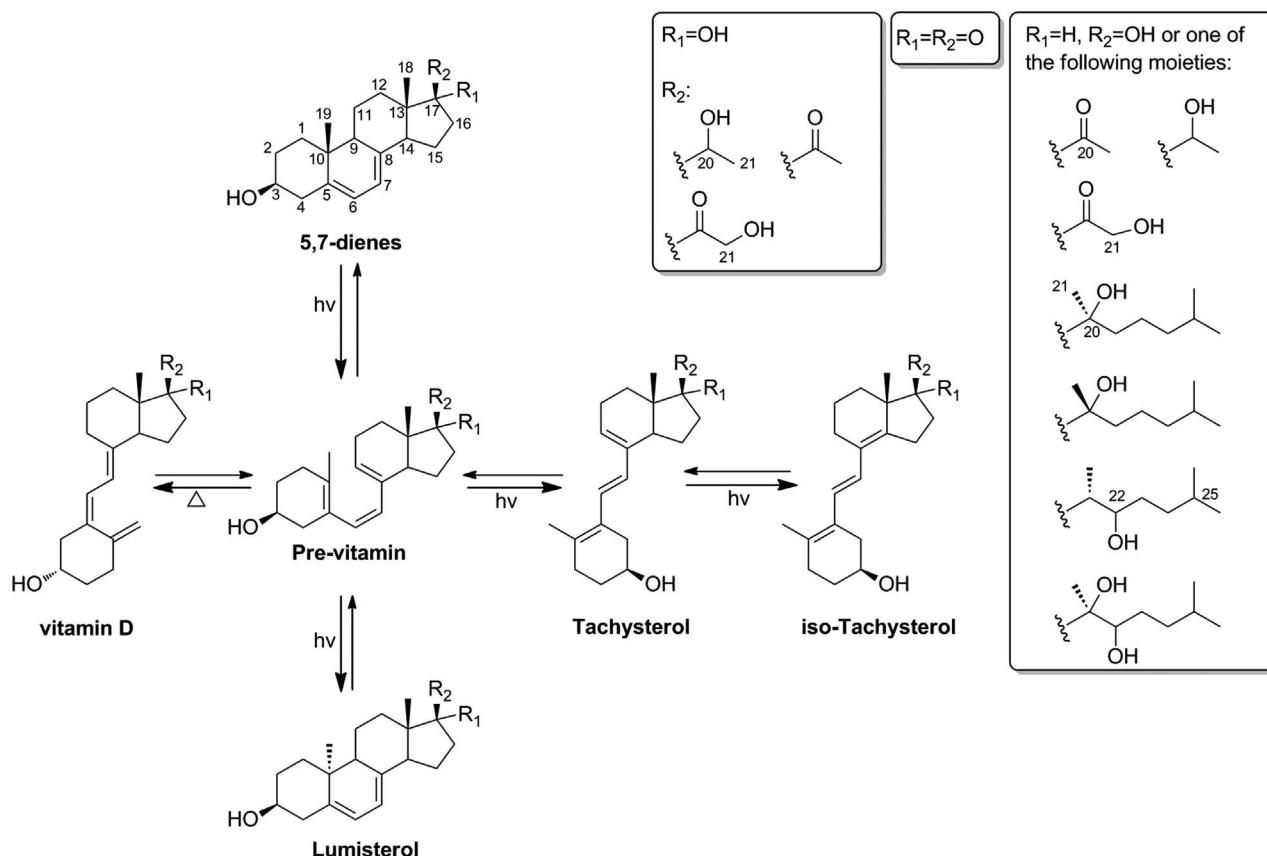
Fig. 3. UVB-induced transformation of steroidal 5,7-dienes with a short or full-length side chain to novel secosteroids.
