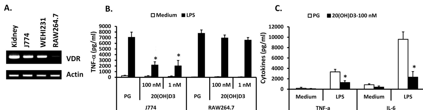
Fig. 4. 20(OH)D3 suppresses TLR4 ligand (LPS)-induced proinflammatory cytokine production in mouse macrophages in a VDR-dependent manner. (A) RT-PCR demonstrates that kidney, J774 cells and WEHI-231 cells express VDR. In contrast VDR mRNA in RAW264.7 cells was only just detectable. The sequences of RT-PCR primers for murine VDR and PCR conditions have been previously described [93]. (B) J774 cells ( 1 \times 10^6 cell/ml) and RAW264.7 cells ( 1 \times 10^6 cell/ml) were pre-treated with vehicle (propylene glycol; PG) or the indicated dose of 20(OH)D3. Forty-eight h later, these cells were stimulated with LPS (25 ng/ml) for 24 h and then TNF \alpha in the culture supernatants was measured by ELISA as described previously [94]. Data represent mean (pg/ml) \pm S.D. of triplicates. LPS-induced TNF \alpha production was significantly suppressed in J774 cells, but not in RAW264.7 cells (** p < 0.005 , * p < 0.05 ). (C) Peritoneal macrophages were isolated from CIA mice (CII-immunized DBA1 mice that fully developed arthritis) as previously described [95]. Peritoneal macrophages ( 1 \times 10^6 cell/ml) were pre-treated with vehicle (PG) or the indicated dose of 20(OH)D3. Forty-eight h later, cells were stimulated with LPS (5 ng/ml) for 24 h and then levels of TNF \alpha and IL-6 in the culture supernatants were measured by ELISA. Data represent mean (pg/ml) \pm S.D. of triplicates. LPS-induced production of TNF \alpha and IL-6 was significantly suppressed by 20(OH)D3 compared to that in vehicle-treated cells (* p < 0.05 ).
