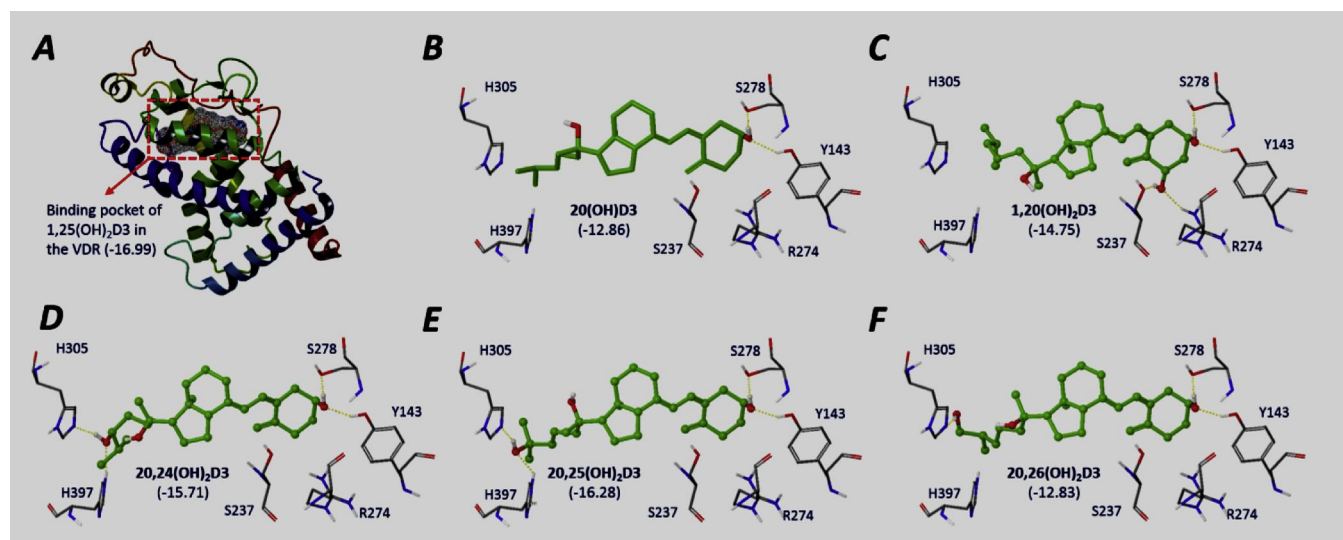
Fig. 5. Potential binding poses of novel secosteroids, docking scores, and hydrogen bonding interactions with the VDR based on molecular modeling. (A) Crystal structure of VDR and its native ligand, 1,25(OH) 2 D 3 . The dotted surface within the rectangle box shows the ligand surface. Docking score (–16.99) is shown in the parenthesis. (B)–(F), predicted binding poses for each of the novel secosteroid in VDR and their hydrogen bonding interactions (dotted line between the atoms in the ligand and the VDR) to the six residues that can form hydrogen bonds to 1,25(OH) 2 D 3 . Molecule modeling studies were performed using the Extra Precision (XP) Glide function within the Schrodinger's Small Molecule Drug Discovery Suite 2012 (Schrodinger Inc., New York, NY, USA). Due to the large number of rotatable bonds in these secosteroids, it is challenging for the software to predict the most favorable binding poses in one run since XP requires a good starting conformation. Thus, for each novel secosteroid, we performed docking calculations iteratively, using the best pose generated from the previous run as the new starting pose for the next run until there was no improvement in the docking score. The optimized docking scores obtained from this process are shown in parenthesis for each panel, along with the predicted hydrogen bonding interactions between the secosteroid and the VDR.
