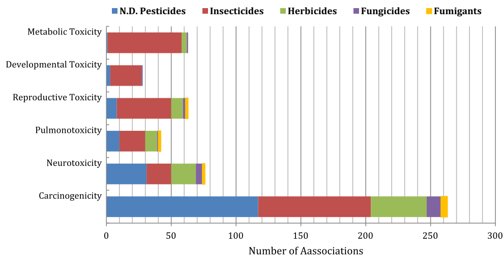
Fig. 2 Schematic diagram showing the weight of evidence on the toxicities of pesticides. ND not determined
